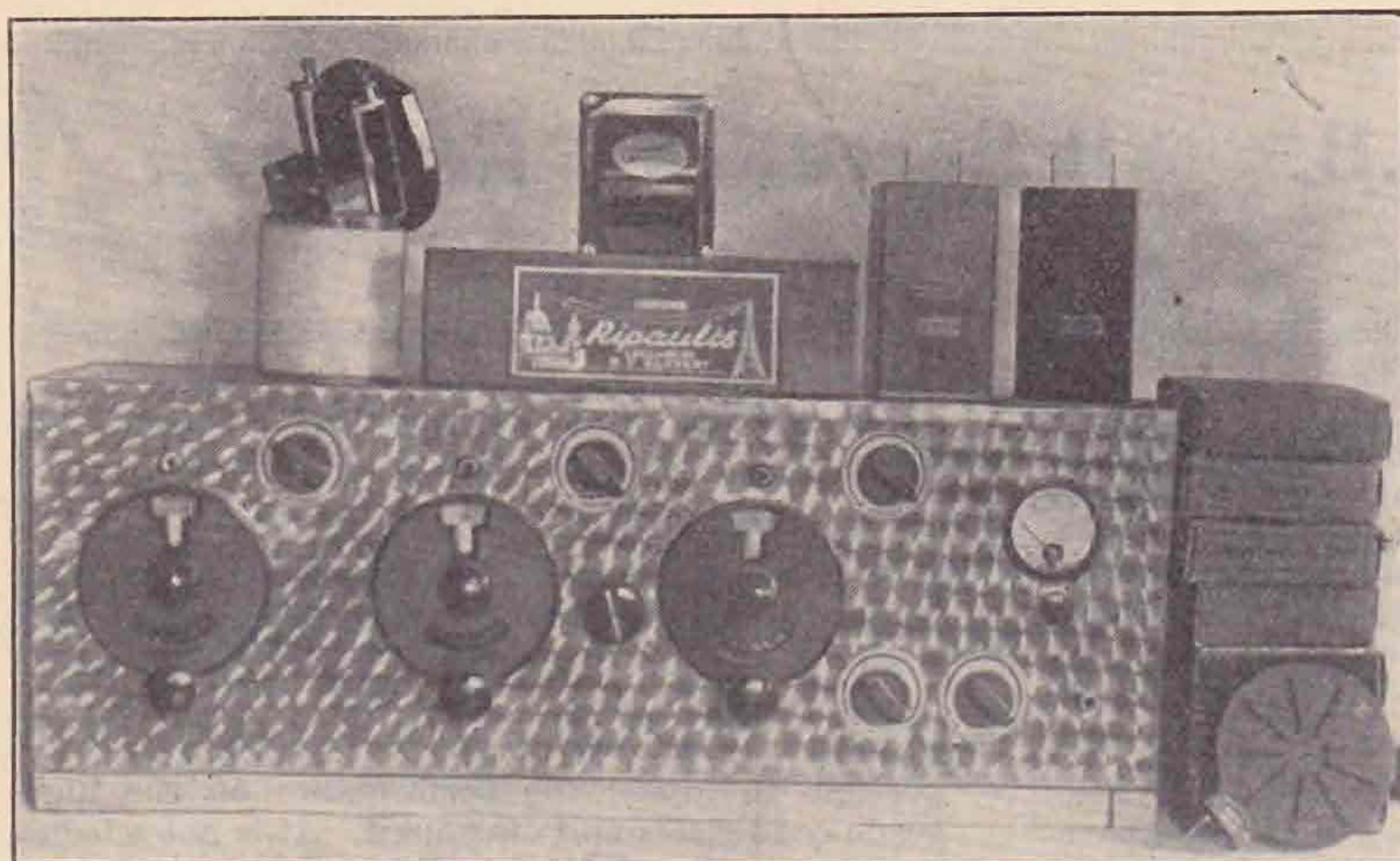
This photograph illustrates the front view of the set and also component parts used exterior to it. These are from left to right, wave-trap inductance and condenser (Ripault). Ripault H.T. battery for use with screened grid valves and as grid bias; Ferranti B1 choke and Dubilier 8 mfd. condensers for coupling loud speaker or head phones to amplifier.
