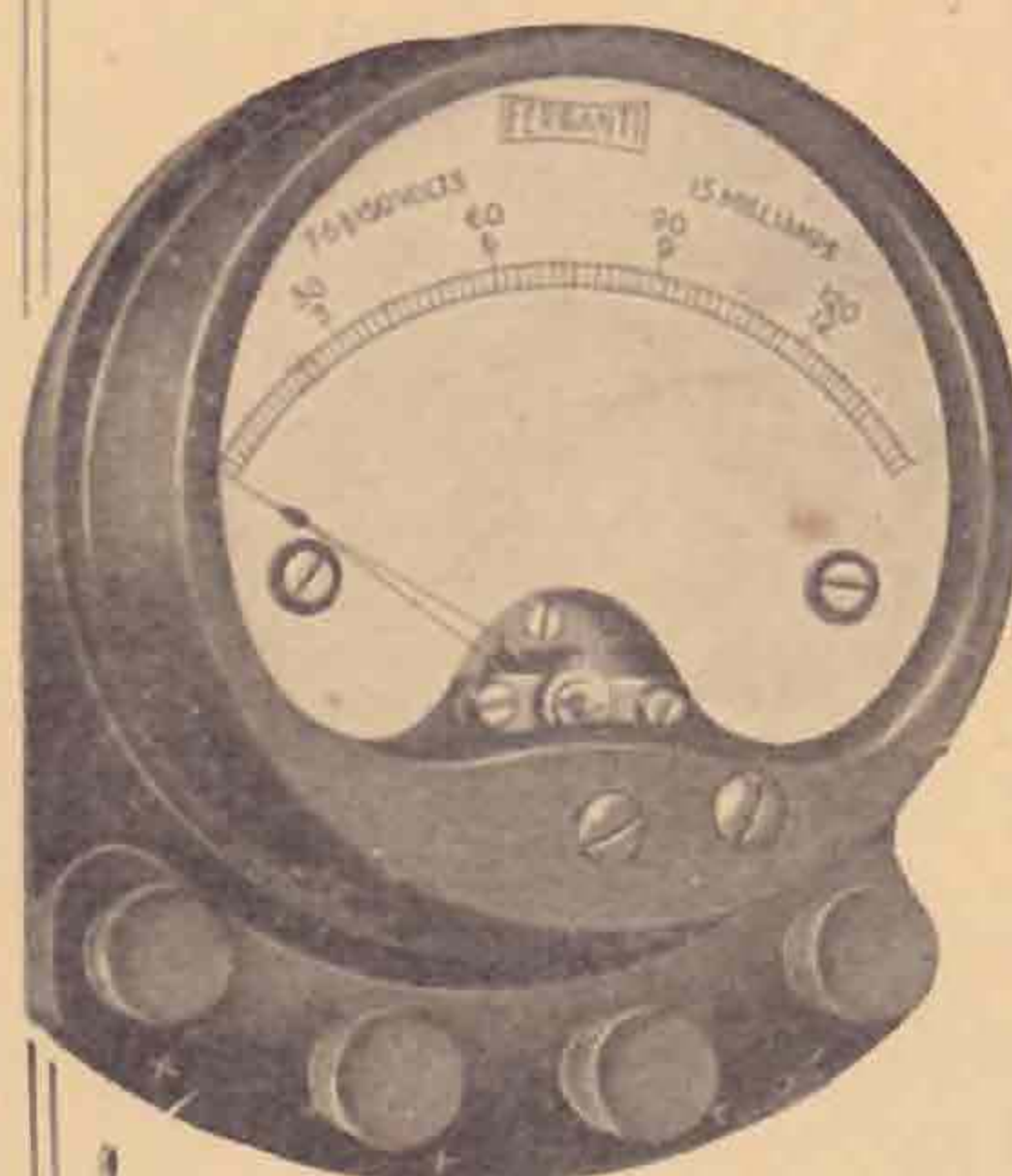
Portable Pattern without Switch Type PR3a.
